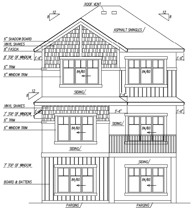
REAR ELEVATION
