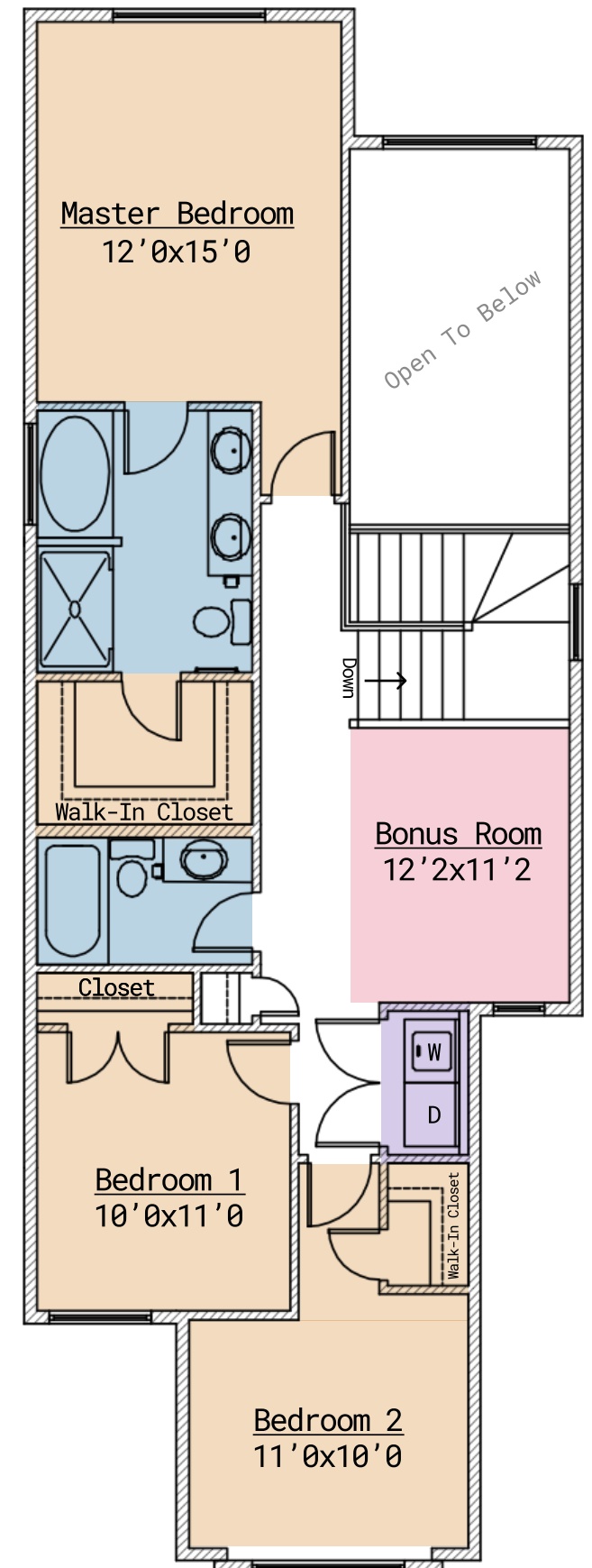
UPPER FLOOR
